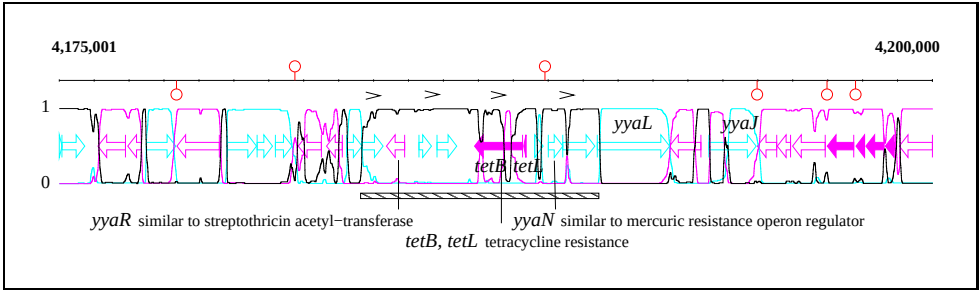
FIG. 3.2 – Detection of an atypical segment (4184-4190 kbp) using a three state M1-M2 model, containing the tetracyclin resistance, and four direct repeats each approximately 100 bp in length, shown by small black brackets.
